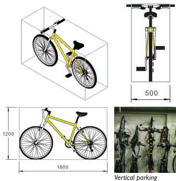
Horizontal parking
